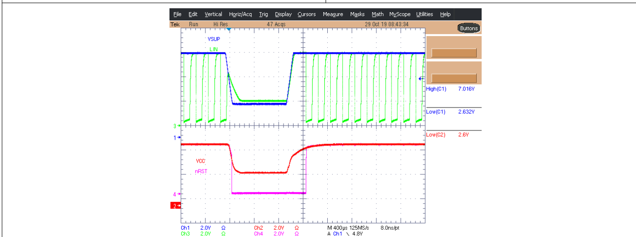
Figure 10-18. TLIN10285-Q1 Brownout
