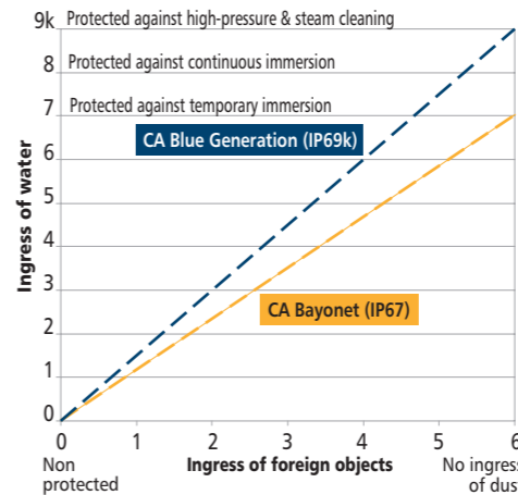
International protection ratings (IP) for IEC 529
