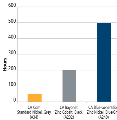
Salt spray resistance with RoHS compliant platings
