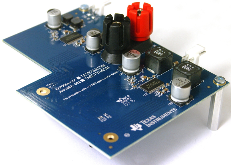
Figure 9. TAS5733LEVM
