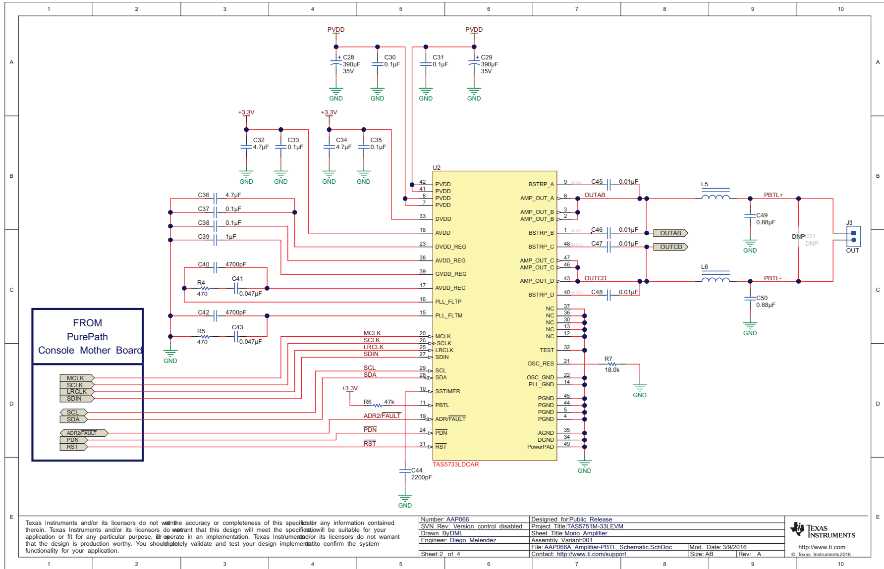
Figure 20. TAS5733LEVM Mono Device
