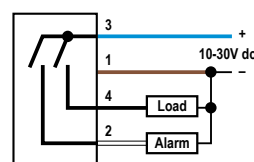
PNP Alarm
