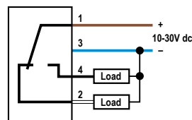
PNP Alarm
