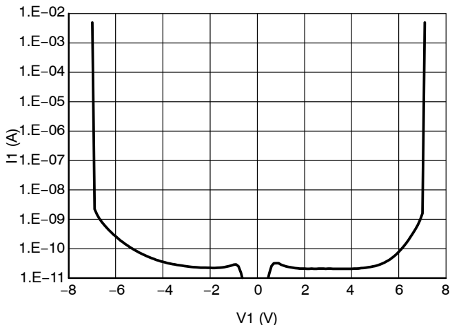
Figure 3. IV Characteristics
