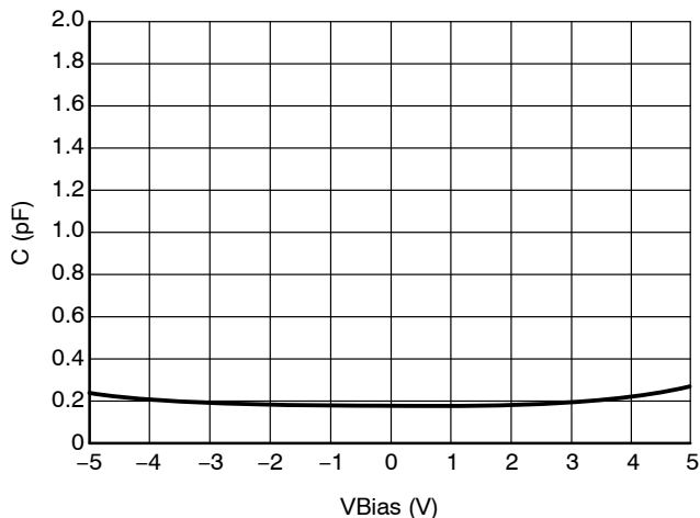
Figure 4. CV Characteristics
