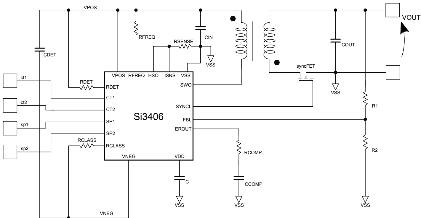
Figure 3.1. Si3406 Non-Isolated Flyback Application Diagram
