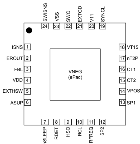
Si34061 Pinout (Top View)
