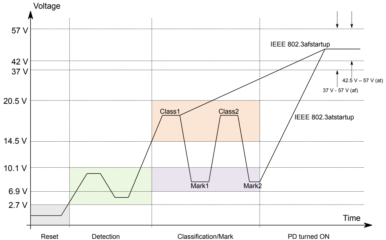
Figure 2.4. Powered Device Voltages
