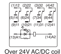
Over 24V AC/DC coil
