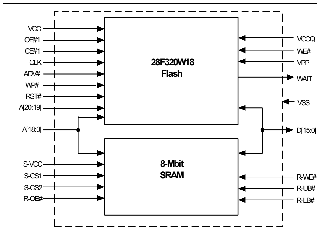
Figure 1. Block Diagram
