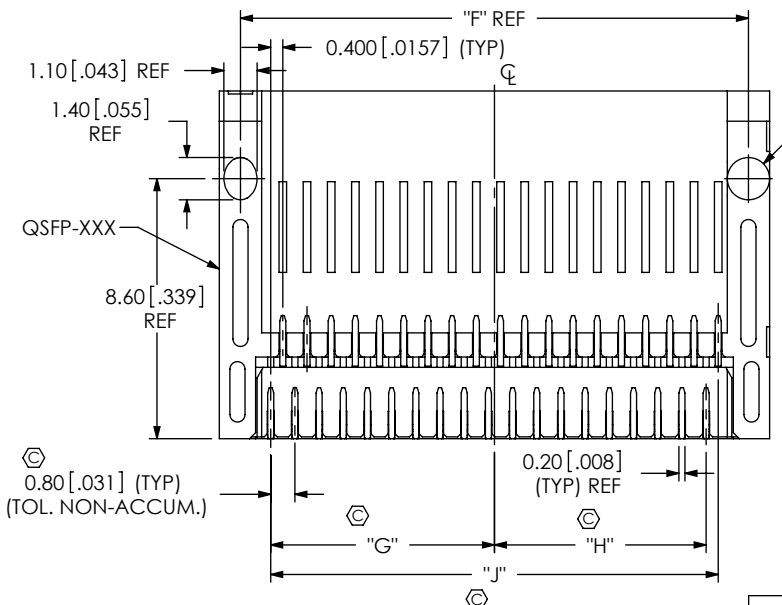
FIG 1 QSFP8-038-01-X-D-RA1 SHOWN SECTION "A"- "A" SCALE 5 : 1
