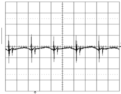
Output voltage ripple (20mV/div.) at: T_{ref} = +25^{\circ}C , I_O = 6 A resistive load, V_I = 12.0 V. Time scale: 2 \mu s/div. See the filter in the Output ripple and noise section (EMC Specification).
