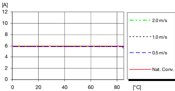
Available load current vs. ambient air temperature and airflow at V_I = 12.0 V, V_{OUT} = 1.8 V . See Thermal Consideration section.
