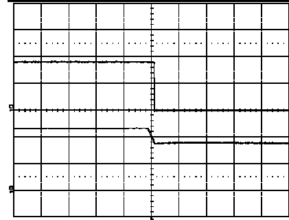
Shut-down enabled by disconnecting V_I at: T_{ref} = +25^{\circ}C , I_O = 6 A resistive load, V_I = 12.0 V. Top trace: output voltage (1.0 V/div.). Bottom trace: input voltage (5 V/div.). Time scale: 10.0 ms/div.
