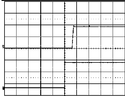
Start-up enabled by connecting V_I at: T_{ref} = +25^{\circ}C , I_O = 6 A resistive load, V_I = 12.0 V. Top trace: output voltage (1.0 V/div.). Bottom trace: input voltage (5 V/div.). Time scale: 20 ms/div.
