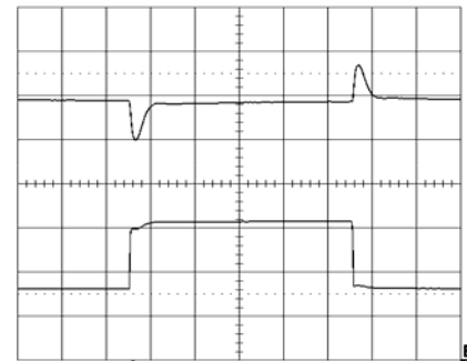
Output voltage response to load current step- change (3-6-3 A) at: T_{ref} = +25^{\circ}C , V_I = 12.0 V. Top trace: output voltage (100mV/div.). Bottom trace: load current (2 A/div.). Time scale: 0.1 ms/div.
