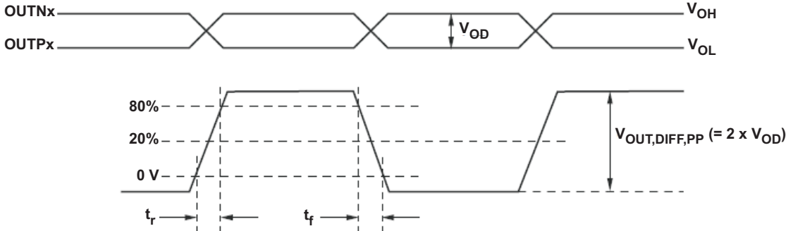
Figure 7. Output Voltage and Rise/Fall Time
