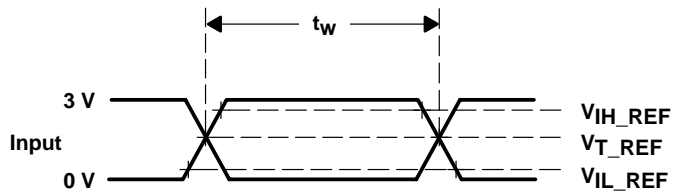
VOLTAGE WAVEFORMS
