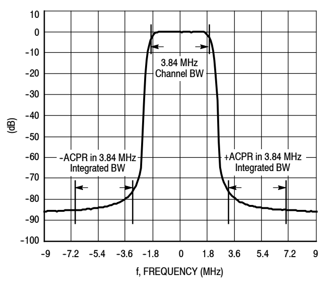
Figure 10. Single-Carrier W-CDMA Spectrum
