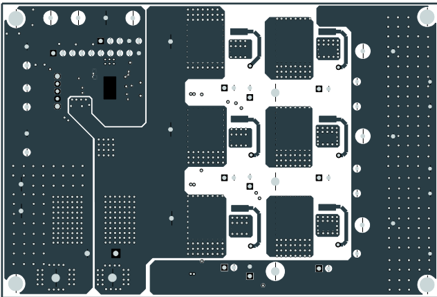
Figure 6: Bottom Layer
