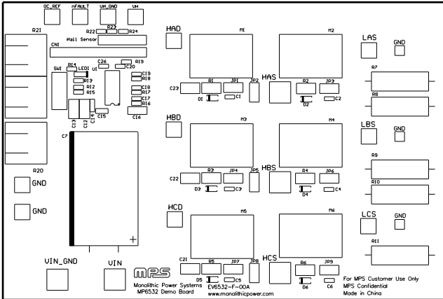
Figure 2: Top Silk
