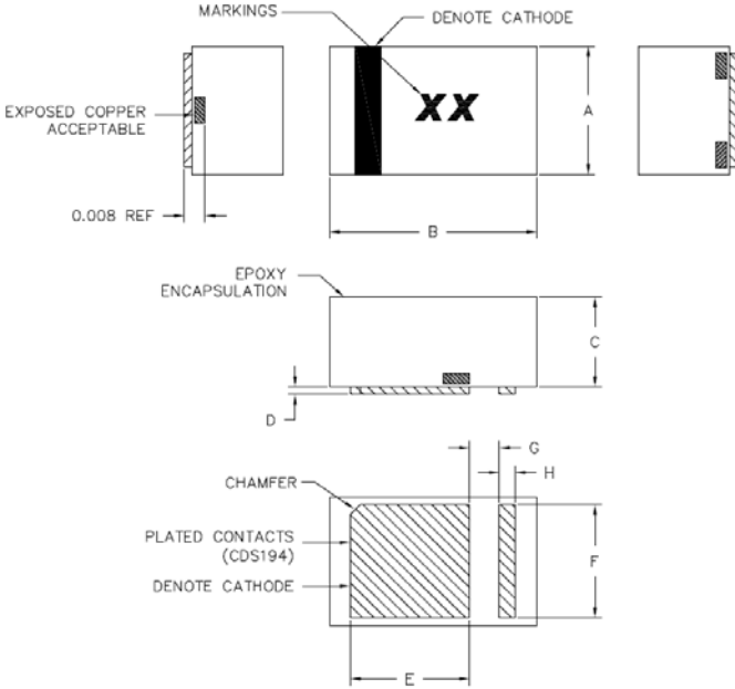
Figure 4 Package Outline
