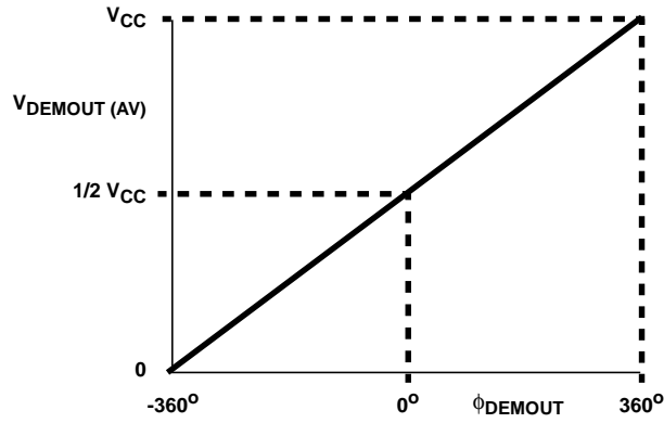
FIGURE 4. PHASE COMPARATOR 2: AVERAGE OUTPUT VOLTAGE vs INPUT PHASE DIFFERENCE: V_{DEMO\text{UT}} = V_{PC2\text{OUT}} = (V_{CC}/\pi) (\phi_{SIG\text{IN}} - \phi_{COM\text{PIN}}) ; \phi_{DEMO\text{UT}} = (\phi_{SIG\text{IN}} - \phi_{COM\text{PIN}})
