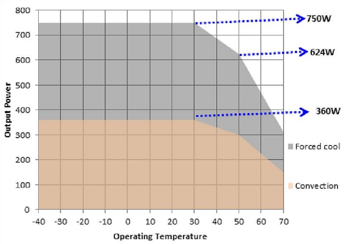
Figure 14. Power Derating Curve 24 V and above with Plain Cover
