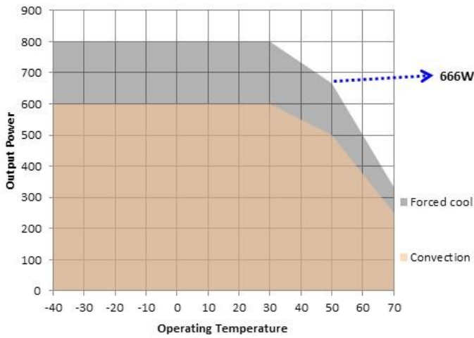
Figure 12. Power Derating Curve 24 V and above
