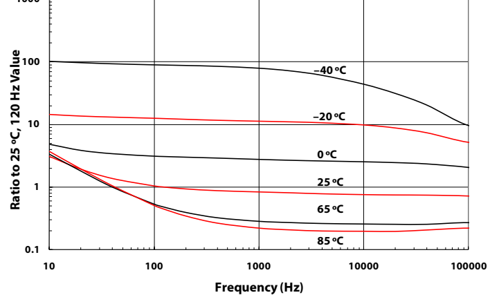
ESR vs Temperature and Frequency, 1300 \mu\text{F} 500 V
