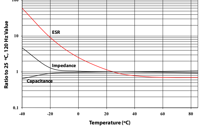
Temperature Characteristics, 4800 \mu\text{F} 200 V
