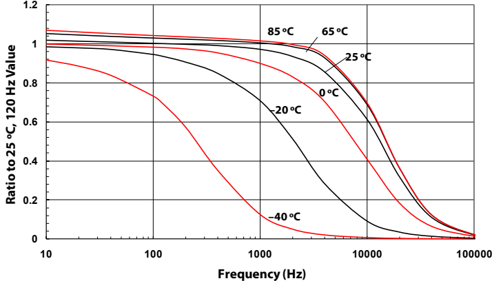
Capacitance vs Temperature and Frequency, 1300 \mu\text{F} 500 V
