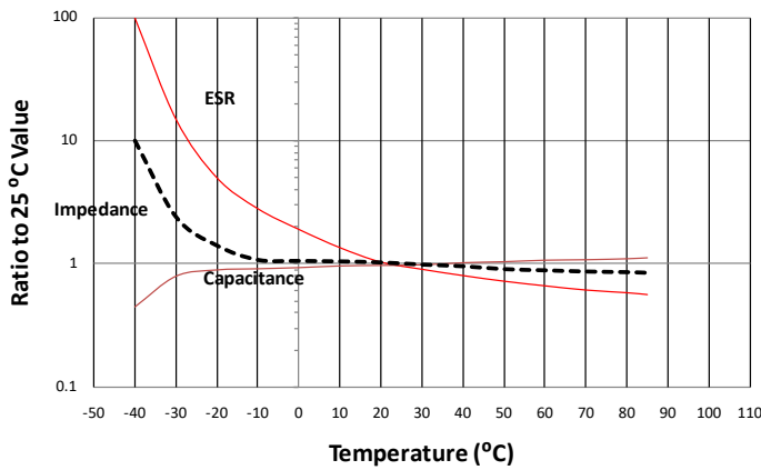
Temperature Characteristics - 29,000 \mu\text{F} 50 Vdc
