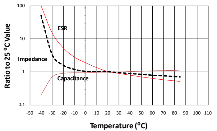
Temperature Characteristics - 100,000 \mu\text{F} 10 Vdc
