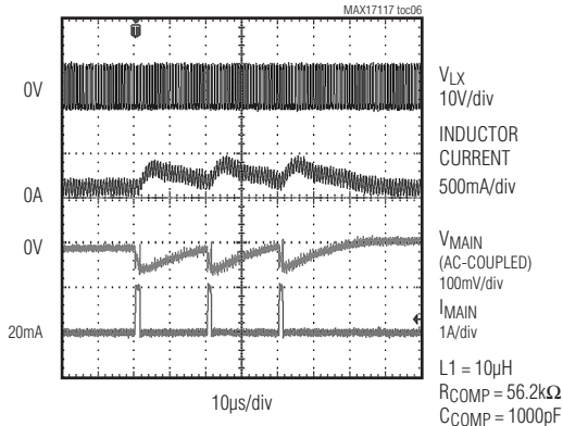
STEP-UP REGULATOR PULSED LOAD-TRANSIENT RESPONSE (20mA TO 1A)
