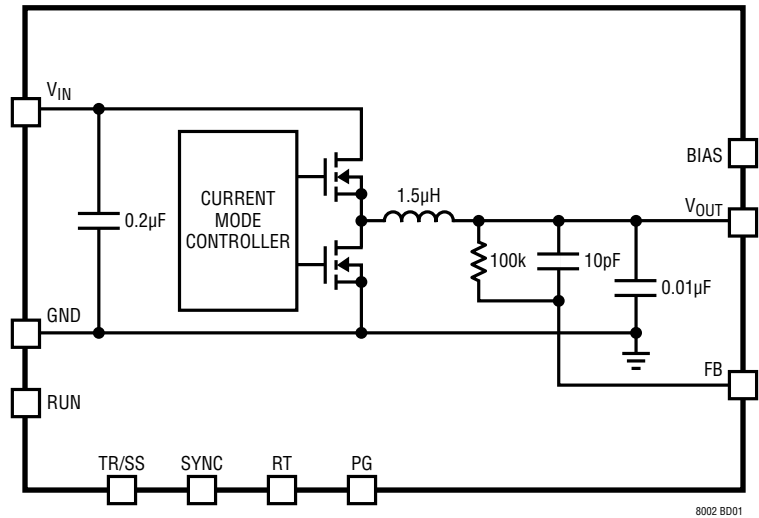
LTM8002 Block Diagram
