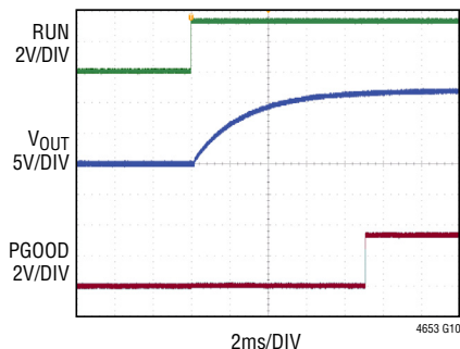
FIGURE 32 CIRCUIT, 48\text{V}_{\text{IN}} , C_{\text{INH}} = C_{\text{D}} = 4.7\mu\text{F} , C_{\text{OUT}} = 22\mu\text{F} \times 2 , R_{\text{ISET}} = 124\text{k} , R_{\text{ISET}} = 240\text{k} , R_{\text{PGDFB}} = 95.3\text{k} , C_{\text{TH}} = 10\text{nF} , R_{\text{TH}} = 562\Omega , R_{\text{EXTVCC}} = 49.9\Omega , C_{\text{EXTVCC}} = 1\mu\text{F} , NO LOAD
