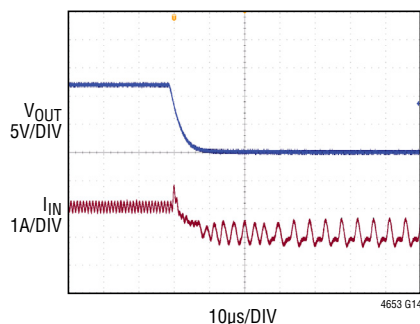
FIGURE 32 CIRCUIT, 48\text{V}_{\text{IN}} , C_{\text{INH}} = C_{\text{D}} = 4.7\mu\text{F} , C_{\text{OUT}} = 22\mu\text{F} \times 2 , R_{\text{ISET}} = 124\text{k} , R_{\text{ISET}} = 240\text{k} , R_{\text{PGDFB}} = 95.3\text{k} , C_{\text{TH}} = 10\text{nF} , R_{\text{TH}} = 562\Omega , R_{\text{EXTVCC}} = 49.9\Omega , C_{\text{EXTVCC}} = 1\mu\text{F} , 3\Omega RESISTIVE LOAD PRIOR TO APPLICATION OF OUTPUT SHORT-CIRCUIT
