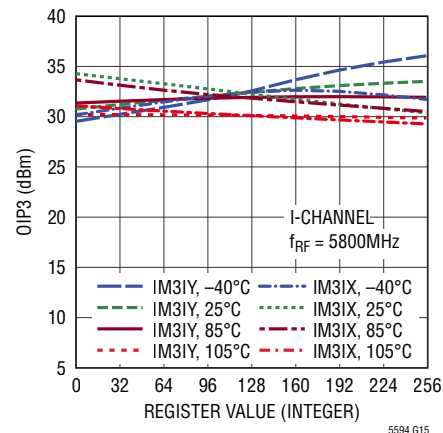
OIP3 vs Temperature ( T_C ) and Register Value
