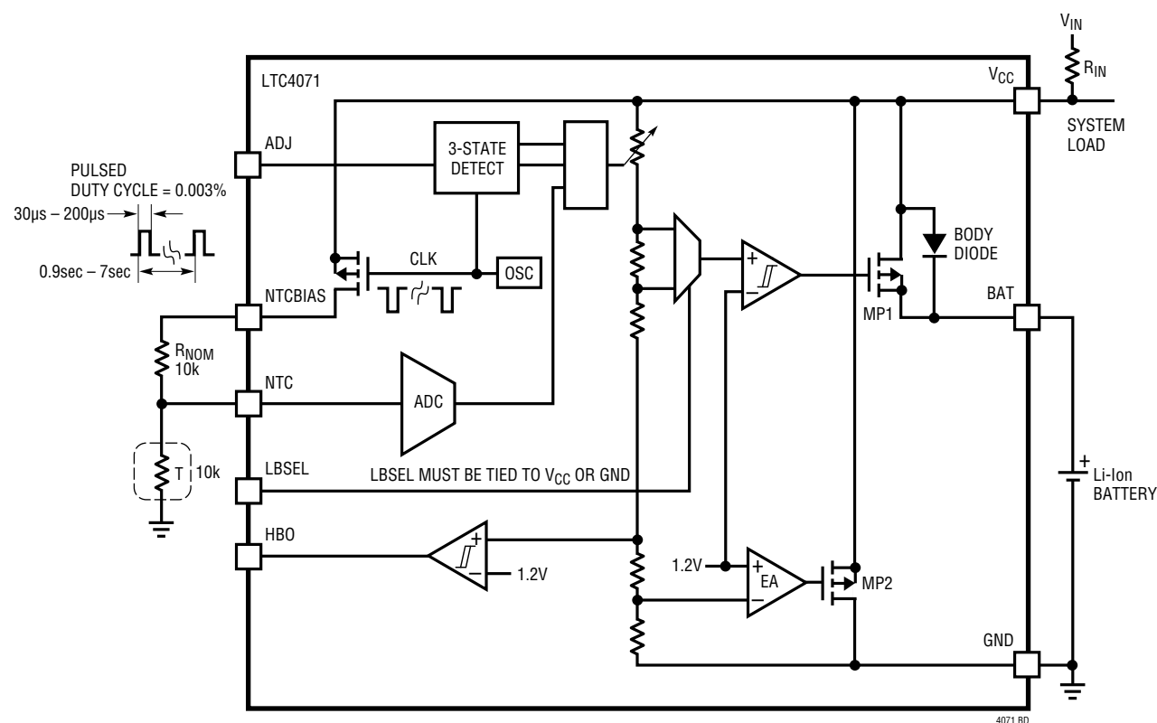
Figure 1. Block Diagram
