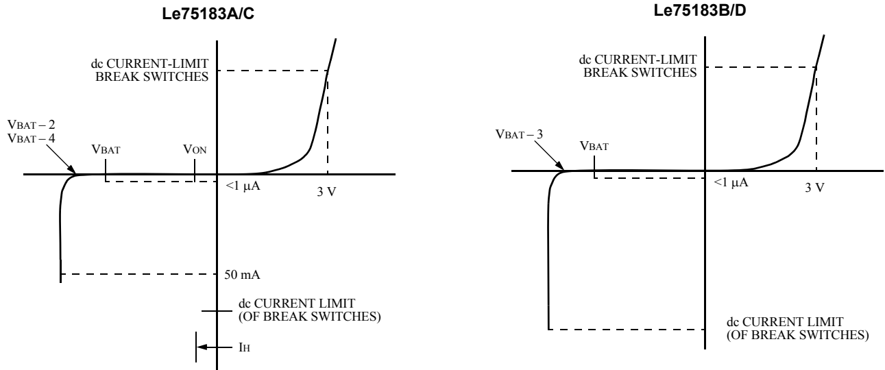
Figure 3. Protection Circuits
