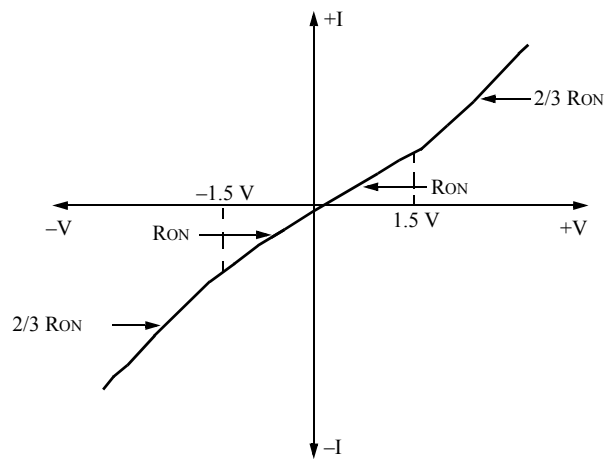
Figure 6. Switches 1, 2, and 5
