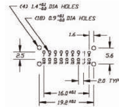
P.C. MOUNTING
