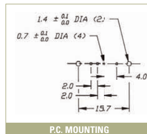
P.C. MOUNTING
