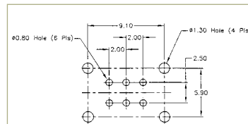
P.C. MOUNTING
