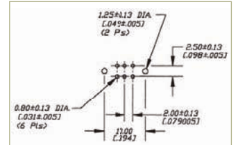
P.C. MOUNTING
