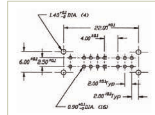
P.C. MOUNTING
