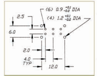
P.C. MOUNTING
