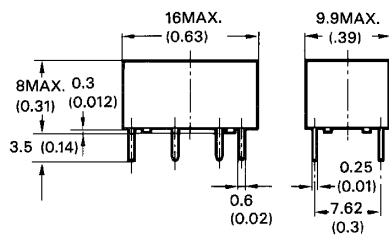
G5A-234P, G5A-234PH, G5A-234P-FC
