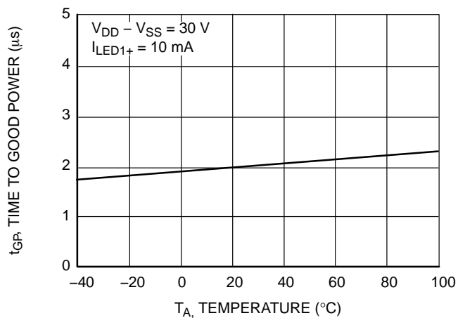
Figure 28. Time-to-Good Power ( t_{GP} ) vs. Temperature
