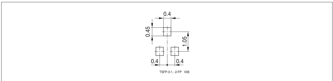
Figure 6-2 PG-TSFP-3-1: Footprint
