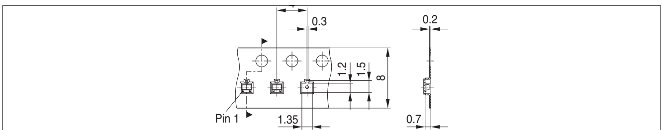
Figure 6-3 PG-TSFP-3-1: Packing
