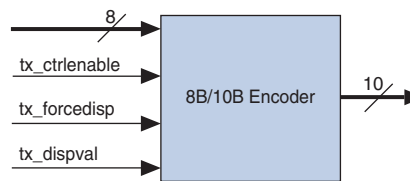
Figure 1-5. 8B/10B Encoder Block Diagram
