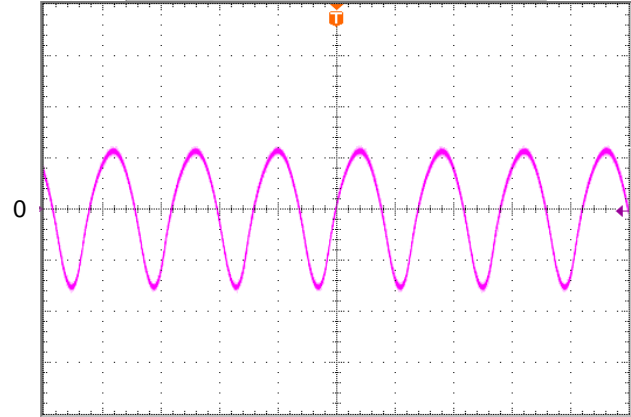
Figure 9: Input Terminal Ripple Current, i_c , at full rated output current and nominal input voltage ( V_{in}=48\text{V} ) with 12 \mu\text{H} source impedance and 33 \mu\text{F} electrolytic capacitor ( 250\text{mA/div} , 2\mu\text{s/div} )
