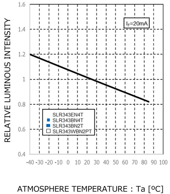
Fig.2 Luminous Intensity -
