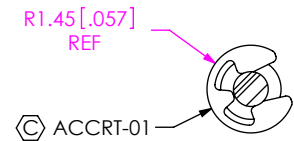
SECTION "C"- "C" SCALE 4 : 1
