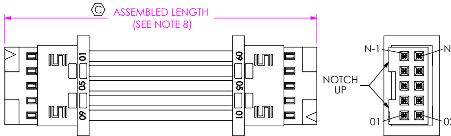
FIG 2 (S2SDX-05-28-X-XX.XX-D-NUS SHOWN) (SAME AS FIG 1, EXCEPT AS SHOWN) (PIN 01 TO N-1)
