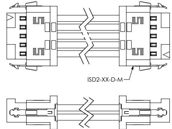
FIG 7 (S2SDX-05-28-X-XX.XX-DR-NUS SHOWN) (SAME AS FIG 6, EXCEPT AS SHOWN)
