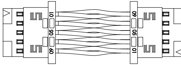
FIG 3 (S2SDX-05-28-X-XX.XX-D-NUX SHOWN) (SAME AS FIG 1, EXCEPT AS SHOWN) (PIN 01 TO N)
