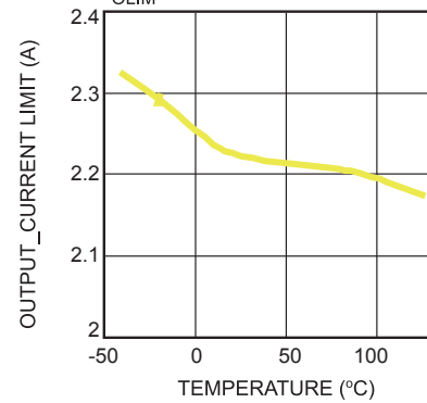
Output_Current_Limit_2.2A vs. Temperature
