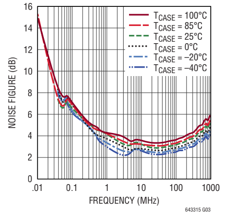
Noise Figure vs Frequency Over Temperature
