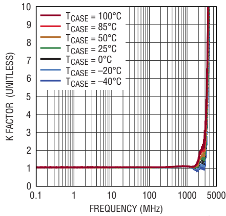
K Factor vs Frequency Over Temperature
