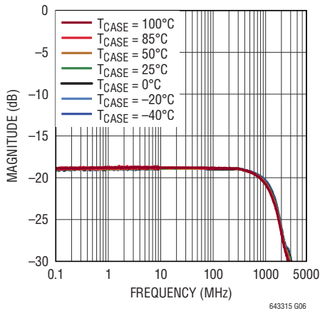
S12 vs Frequency Over Temperature
