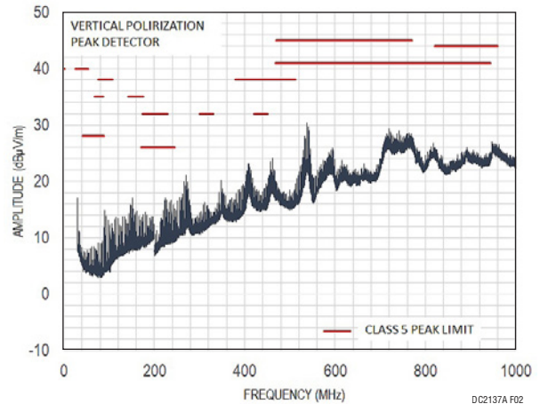
Figure 2. LT8619 DC2137A EMI Performance in CISPR25 Radiated Emission Test (12V Input from V_{EMI} Turret Pin, I_{OUT} = 1A )
