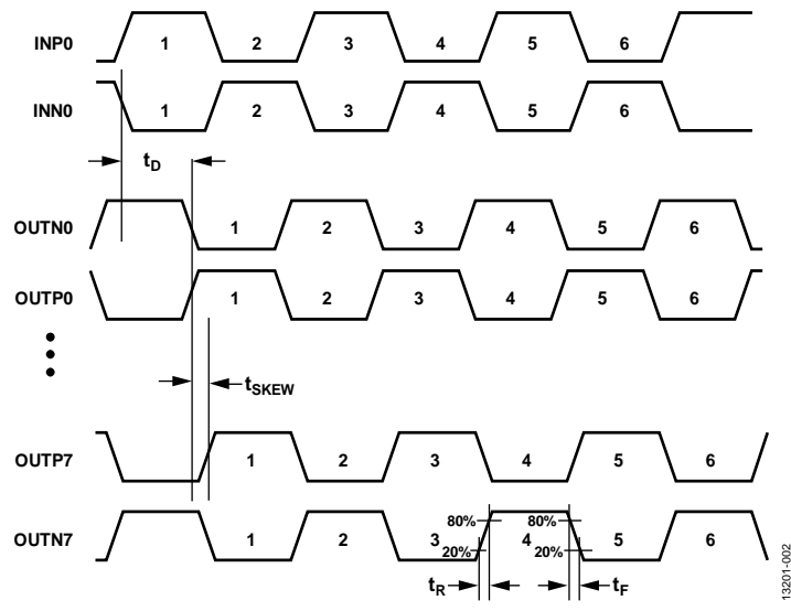
Figure 2. Timing Diagram
