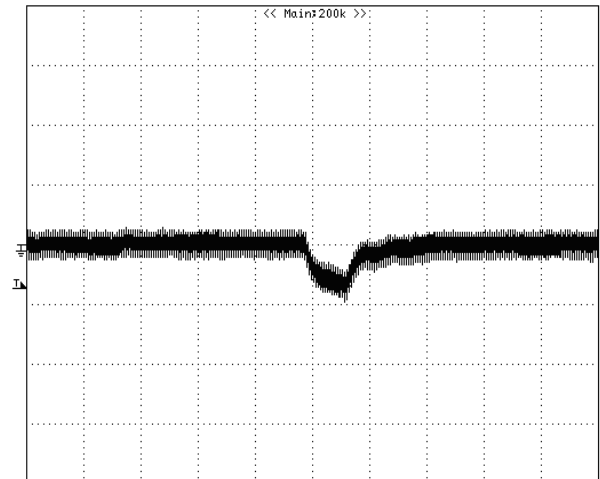
Figure 9: Output voltage response to step-change in load current (50%-75% of I_o , max; di/dt = 0.1A/\mu s ). Load cap: 10\mu F , tantalum capacitor and 1\mu F ceramic capacitor. Trace: V_{out} (50mV/div, 100us/div), Scope measurement should be made using a BNC cable (length shorter than 20 inches). Position the load between 51 mm to 76 mm (2 inches to 3 inches) from the module.
