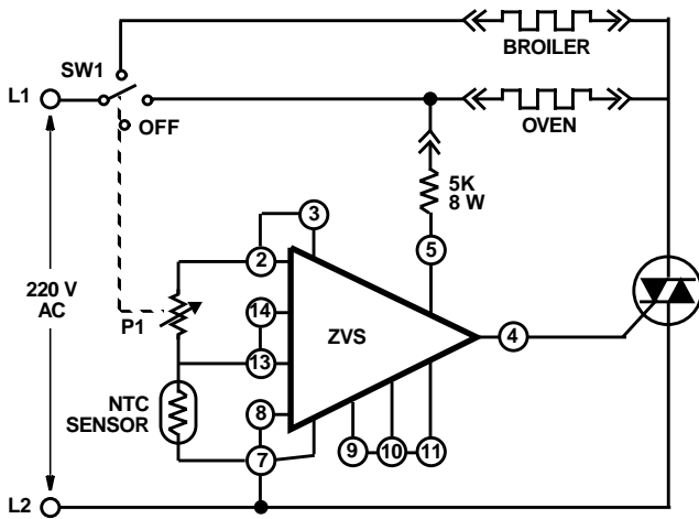
FIGURE 37. SCHEMATIC DIAGRAM OF BASIC OVEN CONTROL Integral Cycle Temperature Controller (No half cycling)
