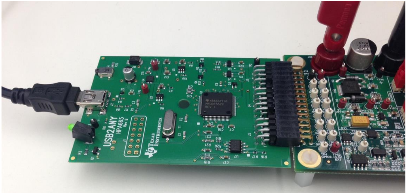
Figure 11. USB2ANY Connection to the PGxxxEVM-034
