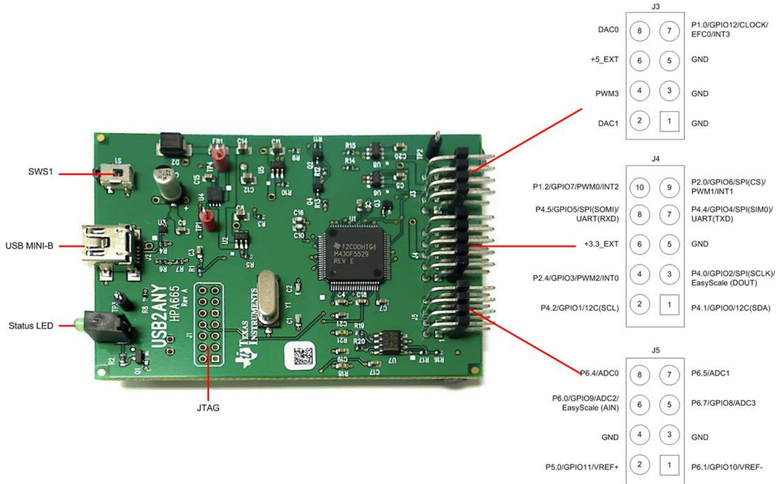
Figure 13. USB2ANY Pinout
