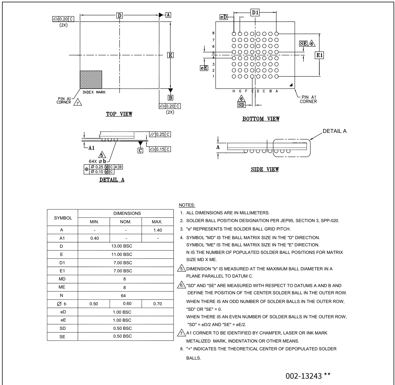
Figure 5 64-ball FBGA (13.0 x 11.0 x 1.4 mm) package outline (PG-LFBGA-64), 002-13243
