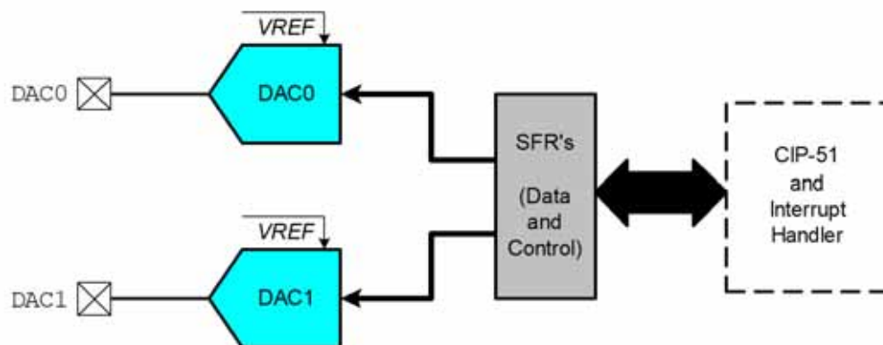
Figure 1.14. DAC System Block Diagram
