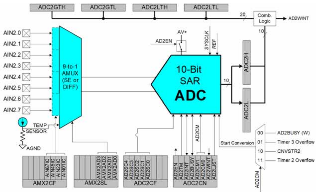
Figure 7.1. ADC2 Functional Block Diagram
