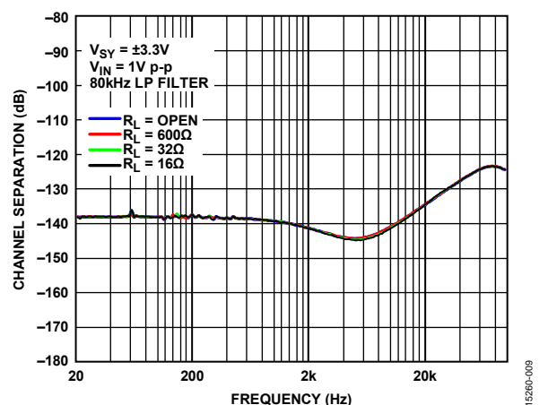
Figure 9. Channel Separation vs. Frequency, V_{SY} = \pm 3.3V
