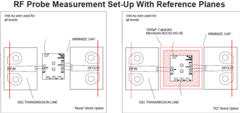
Figure 1 RF Probe Measurement
