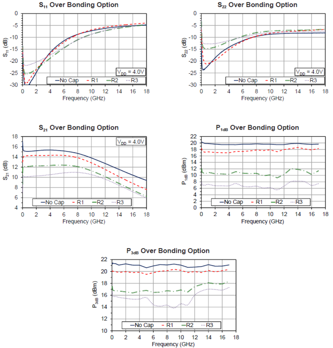
Figure 6 Bonding Option
