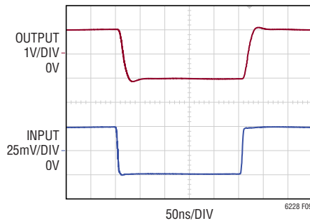
Figure 9. Transient Response
