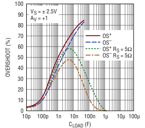
Small Signal Overshoot vs Capacitive Load
