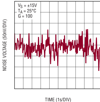
0.1Hz to 10Hz Voltage Noise, G = 100, RTI
