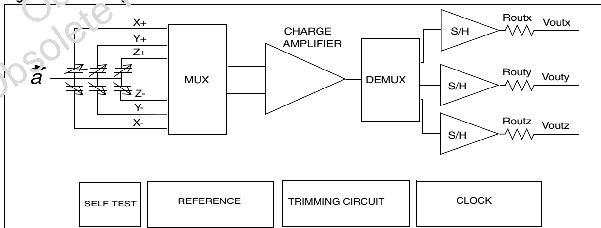
Figure 2. Block Diagram
