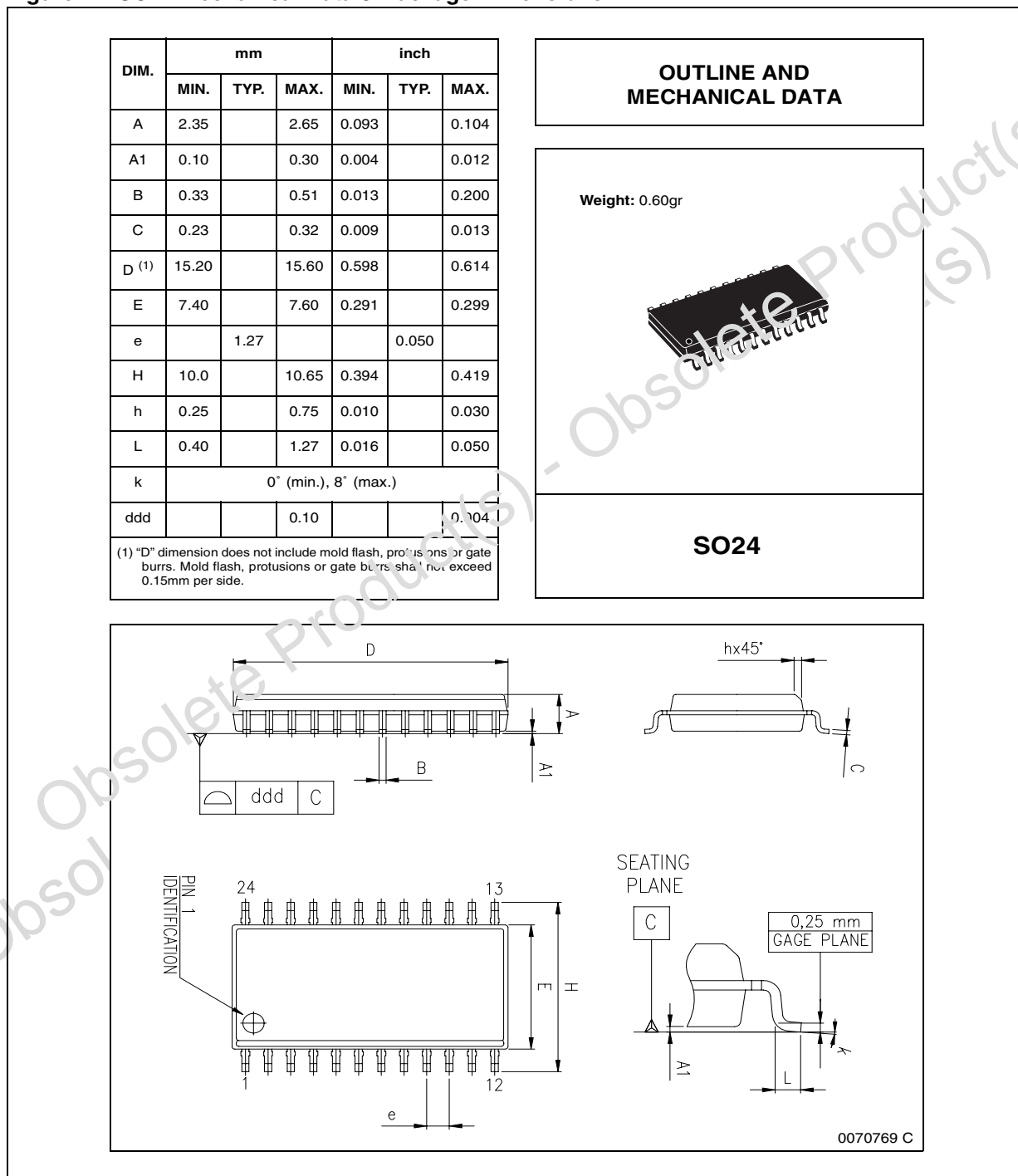
Figure 22. SO24 Mechanical Data & Package Dimensions
