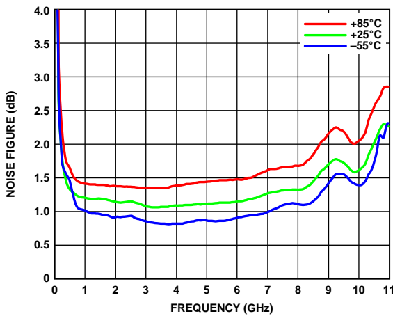
Figure 8. Noise Figure vs. Frequency for Various Temperatures
