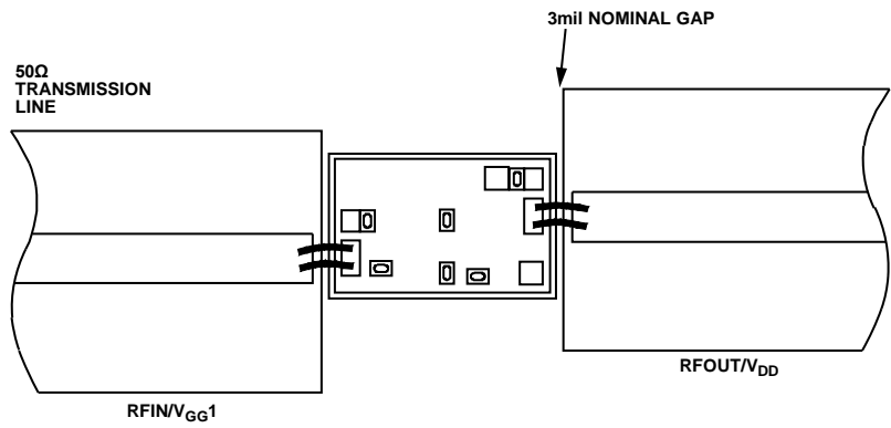
Figure 41. Assembly Diagram
