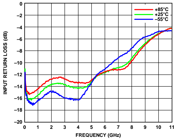
Figure 7. Input Return Loss vs. Frequency for Various Temperatures
