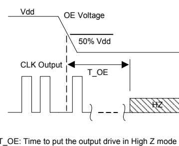
Figure 5. OE Disable Timing (OE Mode Only)
